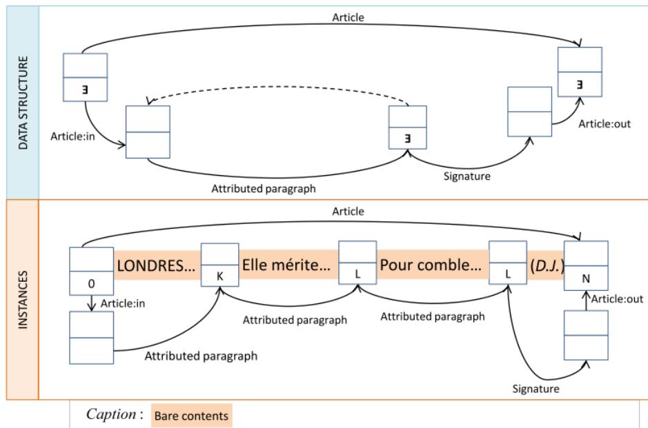
Figure 2: The structure states that an article contains one or more “Attributed paragraph”, and one “Signature”. The \exists symbol indicates that a corresponding node in the instances should be indexed. An instance of that is illustrated underneath. The bare contents are not included in the instance graph, since contents are referred to by the indexes on the nodes of the graph.
